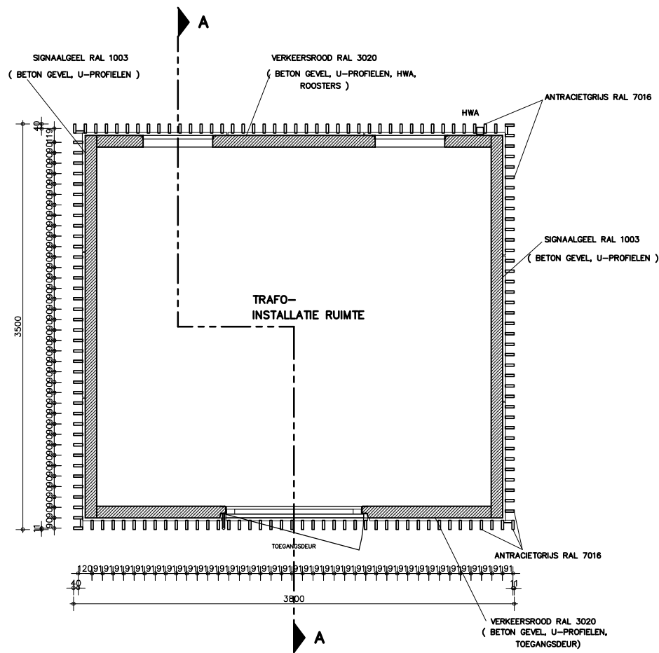
PLATTEGROND TRANSFORMATORSTATION
